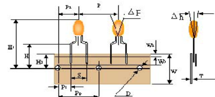
Dimension of tape and reel(Per specification IEC286-2)
